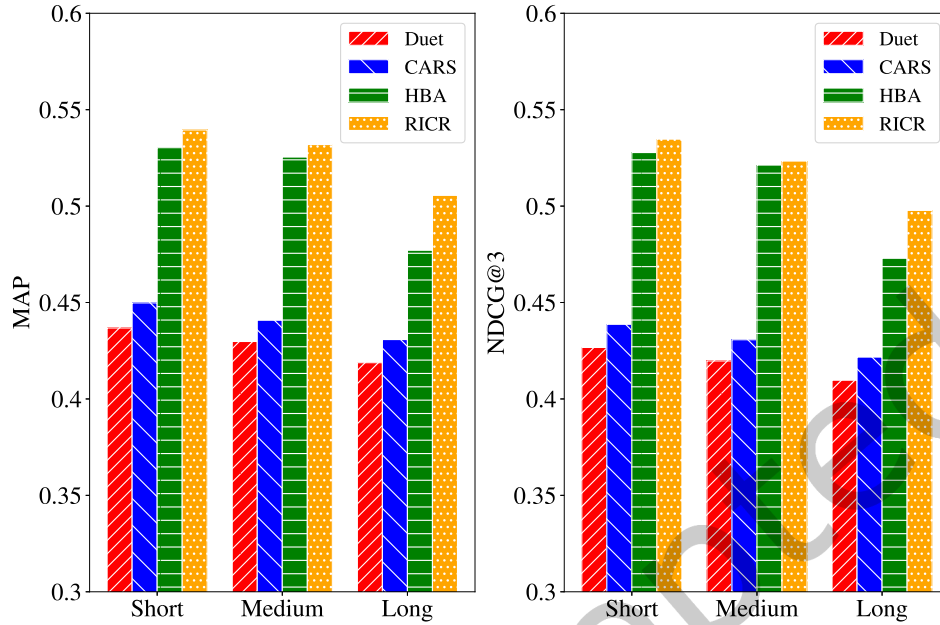
Fig. 3. Performance on sessions with different lengths.
