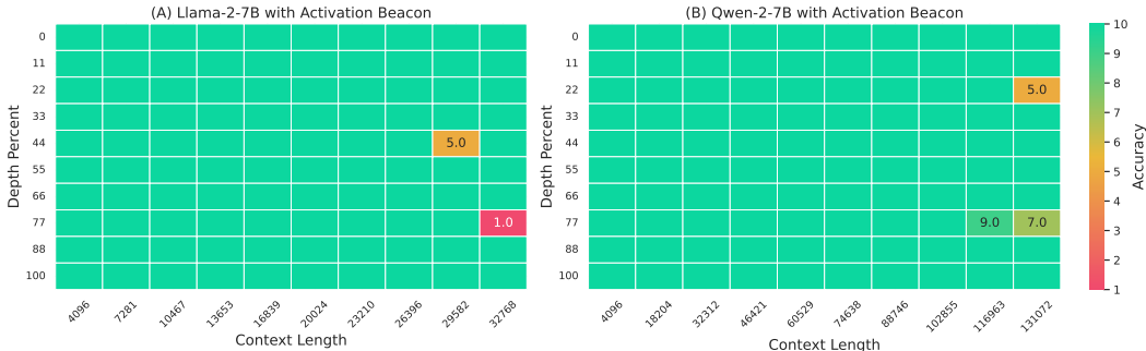
Figure 4: Evaluation on Needle-in-a-Haystack. Activation Beacon can accurately retrieve the needle most of the time, despite the context is far longer than its training data.
