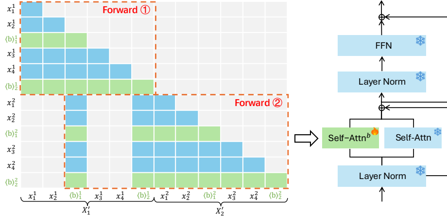
Figure 2: Activation Beacon performs compression during self attention while reusing all other modules of the LLM. Forward ① : encode and compress the first chunk. Forward ② : encode and compress the second chunk conditioned on activations of preceding beacon tokens.
