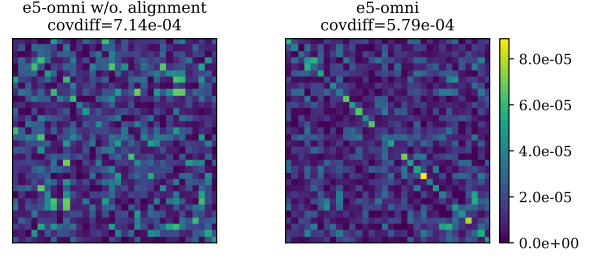
Figure 4: Covariance-difference heatmap on VOC2007. Left: e5-omni w/o. alignment. Right: e5-omni. After a fixed 32D random projection, we visualize covdiff : the entrywise magnitude of the query–target covariance difference matrix.
